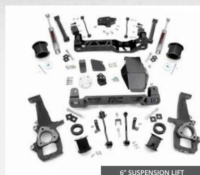
6" SUSPENSION LIFT
