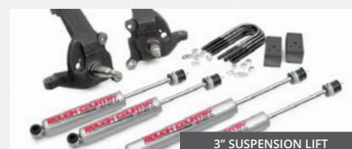
3" SUSPENSION LIFT
